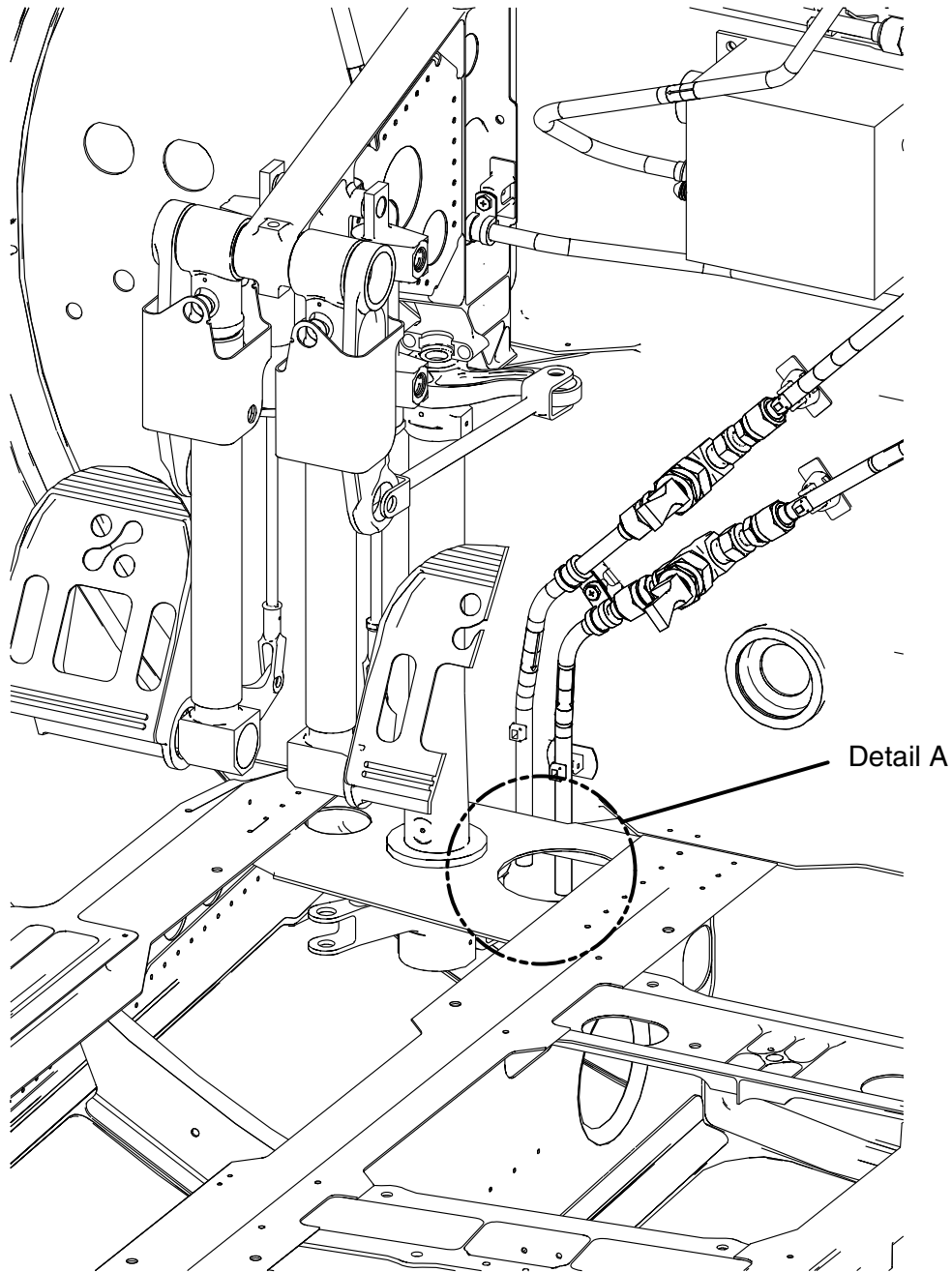
Static Drain Lines Figure 1
